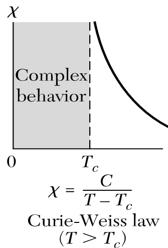
Ferromagnetism
