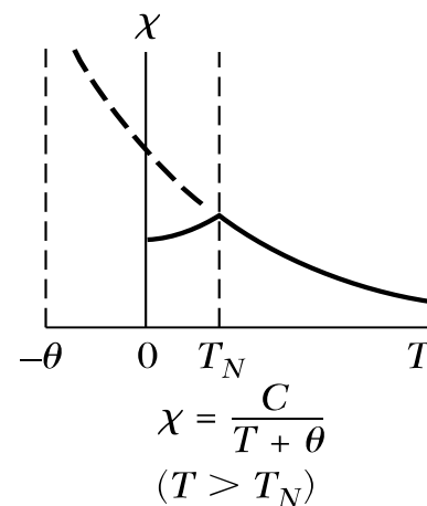
Antiferromagnetism
